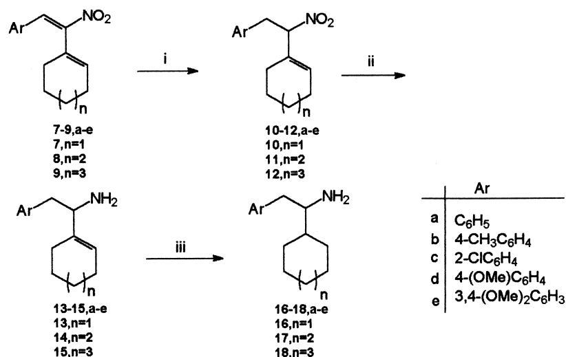
Scheme 2. Synthesis of 1-amino-1-cycloalkyl-2-substituted phenyl ethanes. Reagents and conditions: (i) NaBH 4 , MeOH, 30 min; (ii) Raney-Ni/H 2 , MeOH, 4.5 kg/cm 3 , 3–4 h; (iii) 10% Pd-C/H 2 , MeOH, 4.5 kg/cm 3 , 24 h.
